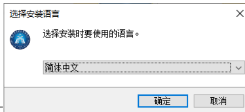
A320CL.exe
